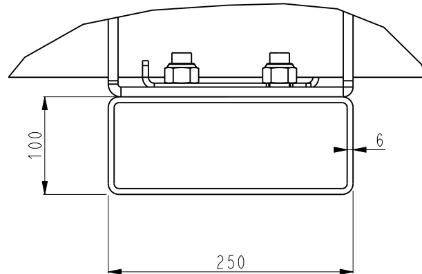
DETAIL C ECHELLE 3:16 SCALE
