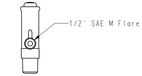
DETAIL SOUPAPE 9
