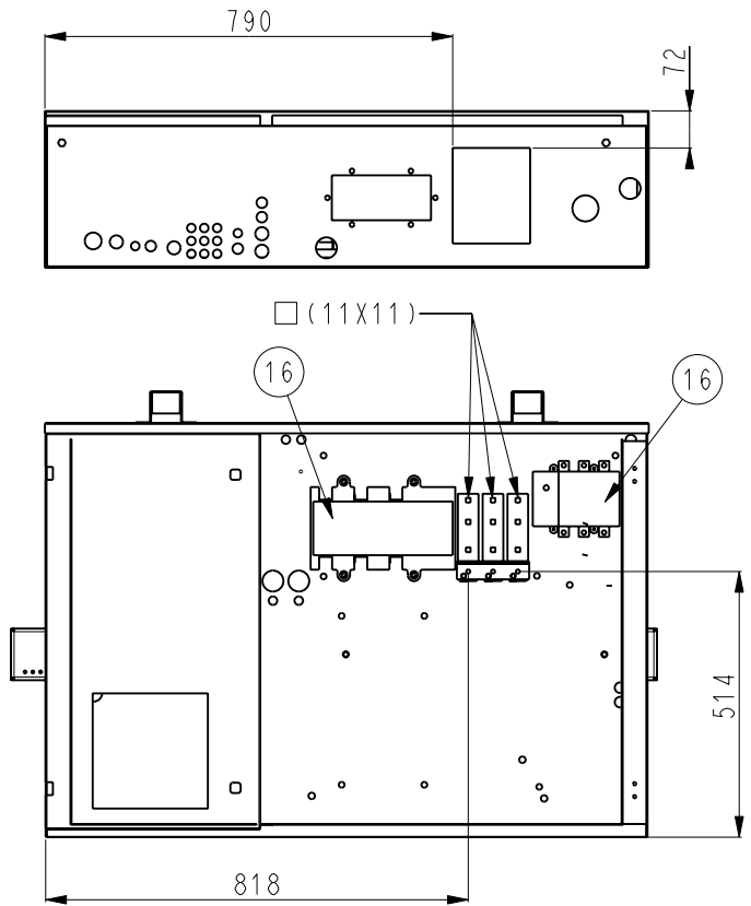
ELECTRICAL BOX: POWER CONNECTION
