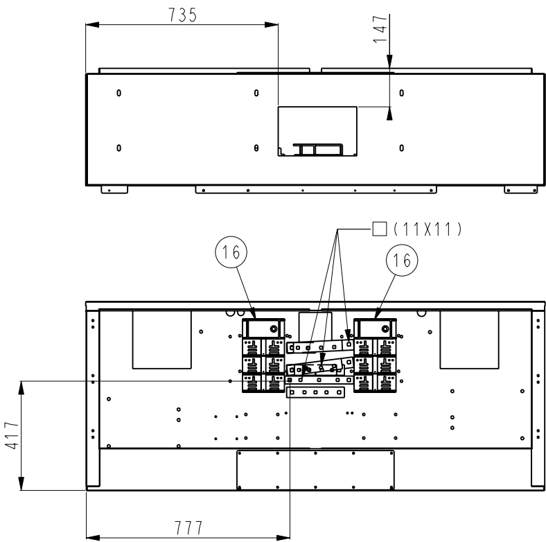
ELECTRICAL BOX: POWER CONNECTION
