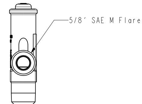
DETAIL SOUPAPE 5
