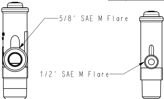
DETAIL SOUPAPE 5
