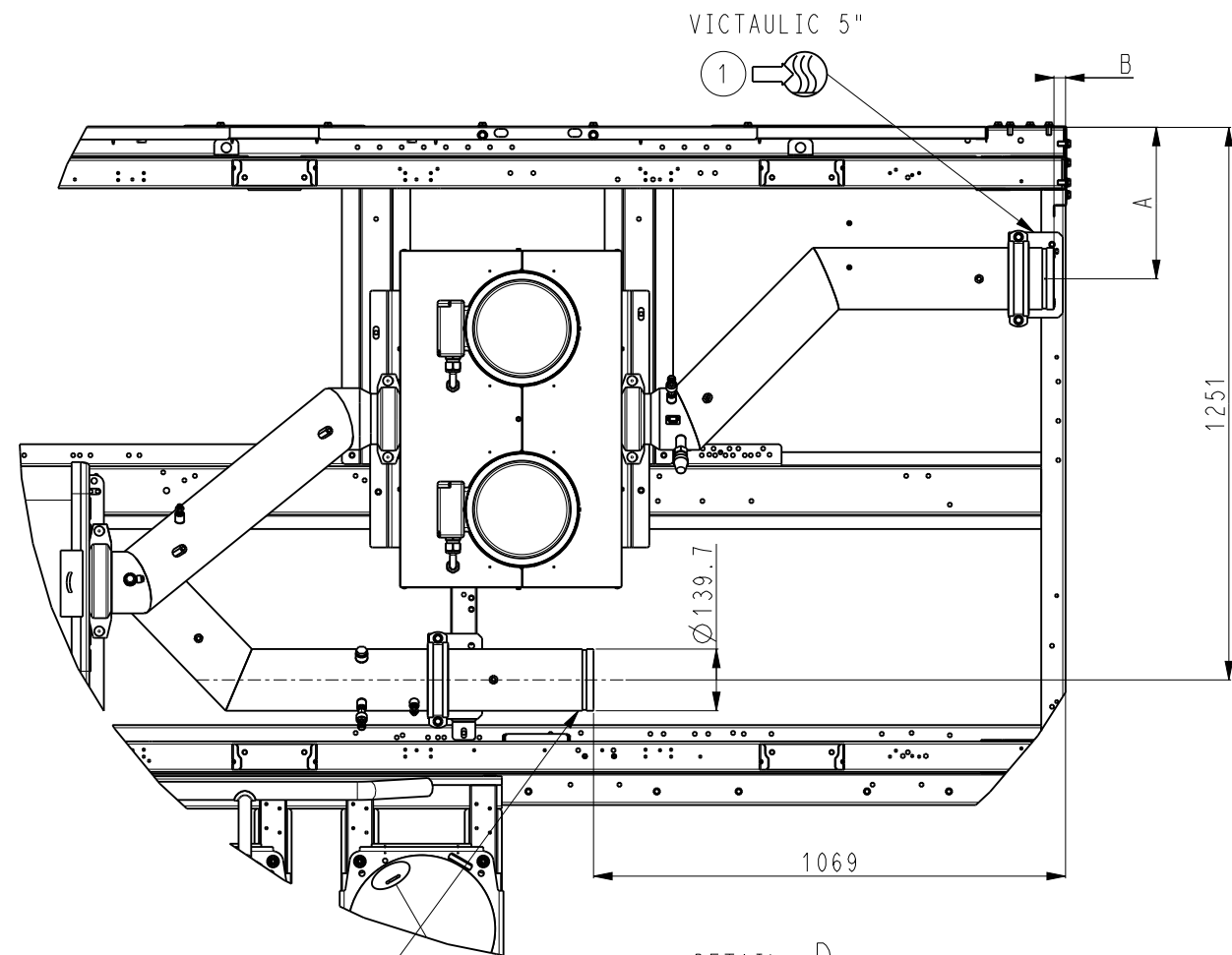
DETAIL D ECHELLE 19:320
