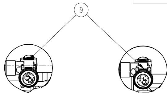
DETAIL C ECHELLE 3:10
