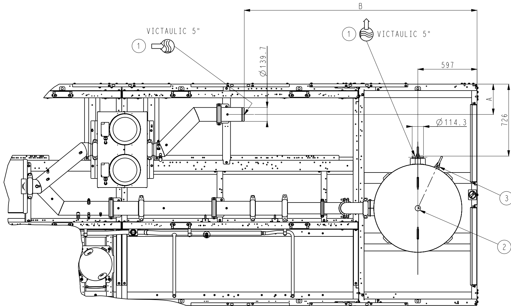
DETAIL C ECHELLE 7:160
