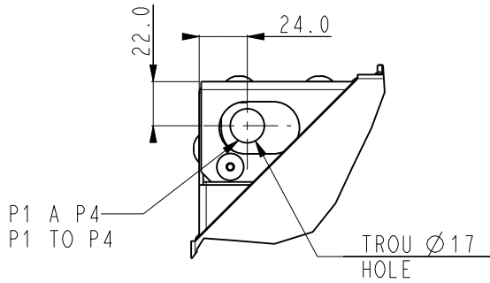
DETAIL C ECHELLE 3:10
