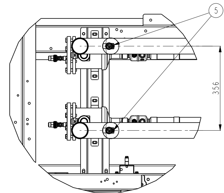
DETAIL B ECHELLE 1:10
