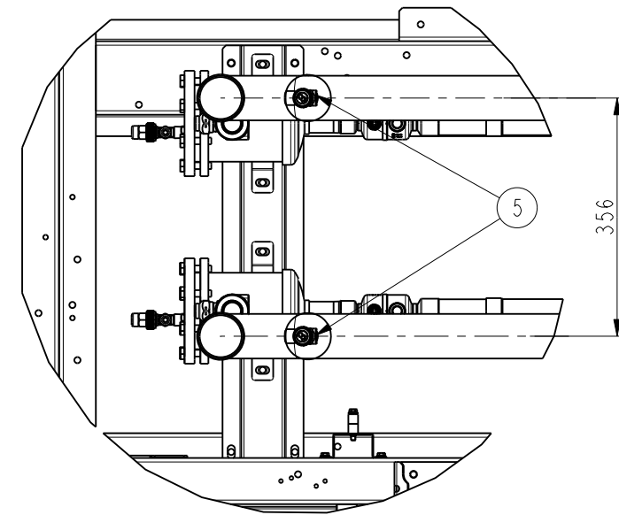
DETAIL B ECHELLE 1:10
