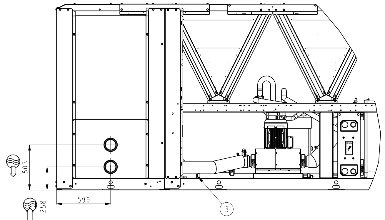
DETAIL B ECHELLE 1:10
