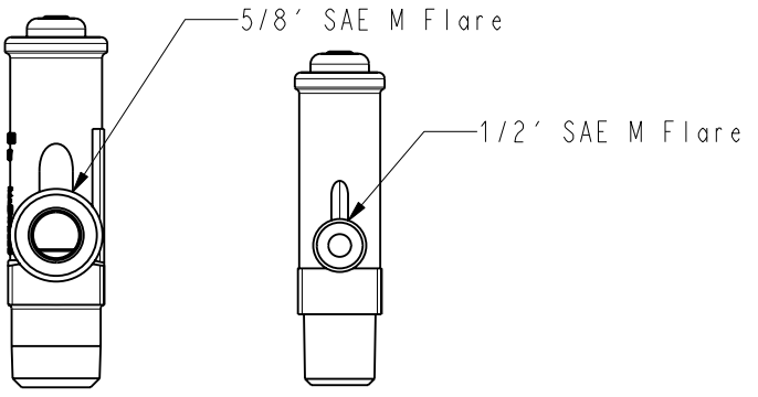
DETAIL SOUPAPE 5 DETAIL SOUPAPE 9
