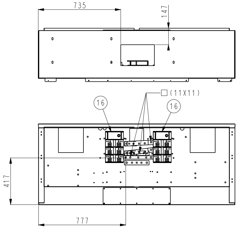
A400 30XBE0850/0900 ELECTRICAL BOX: POWER CONNECTION
