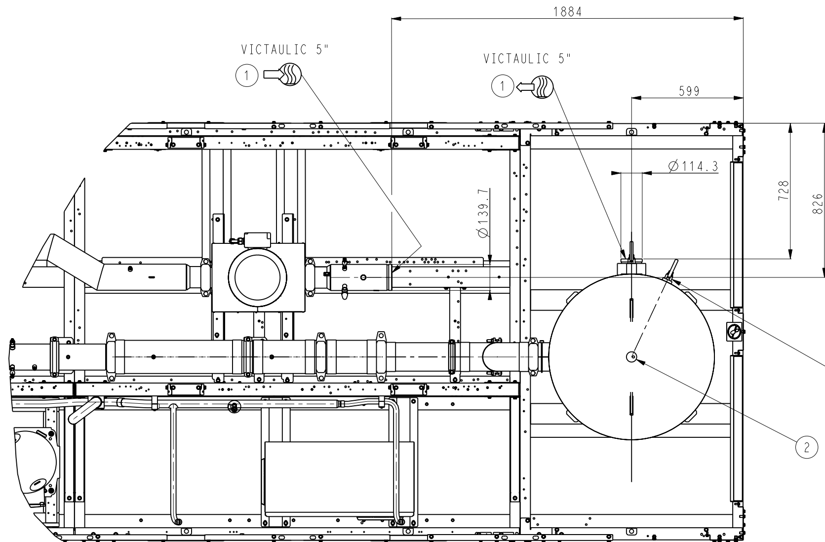
DETAIL F ECHELLE 1:20
