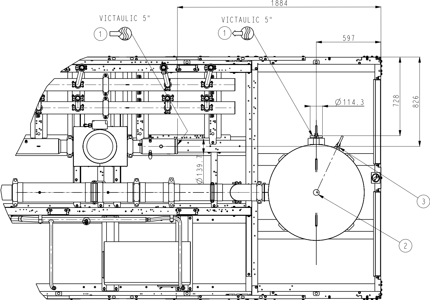
DETAIL E ECHELLE 1:20
