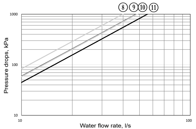
Sizes 610R - 950R
