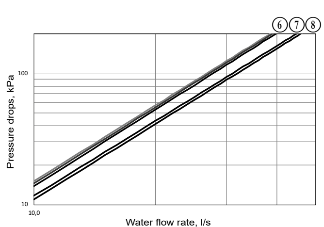
Sizes RBP 450R - 950R
