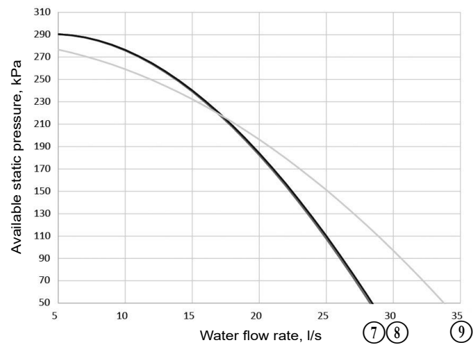
Sizes 610R - 950R
