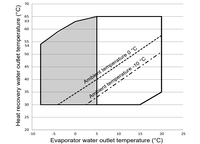
Operating range in heat recovery mode
