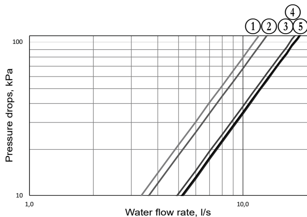
Sizes RBP 170R - 410R
