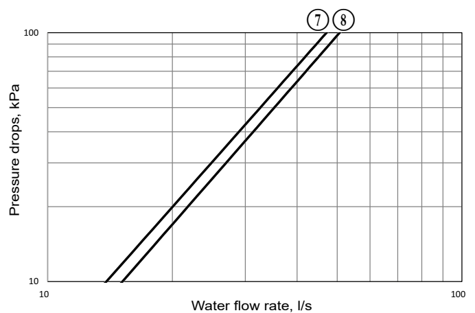
Sizes 610R - 950R
