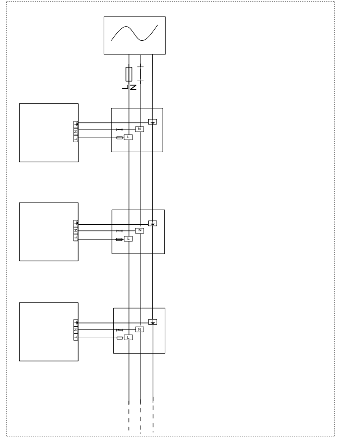
Correct wiring for several units
