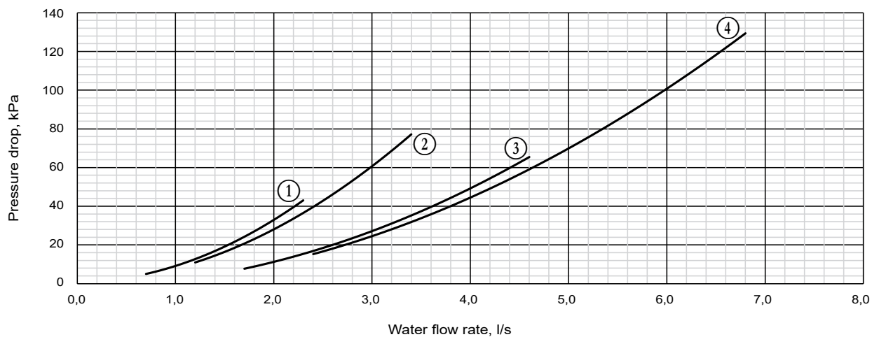
Water pressure drop in the unit
