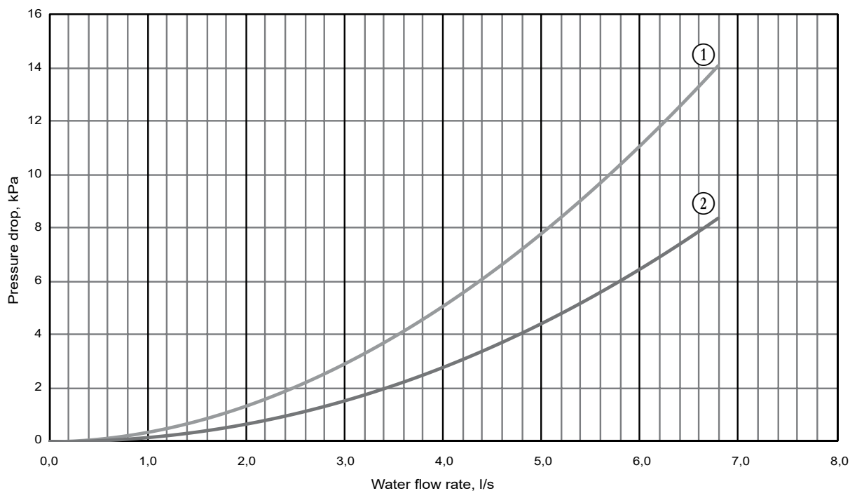
Water pressure drop in the filter
