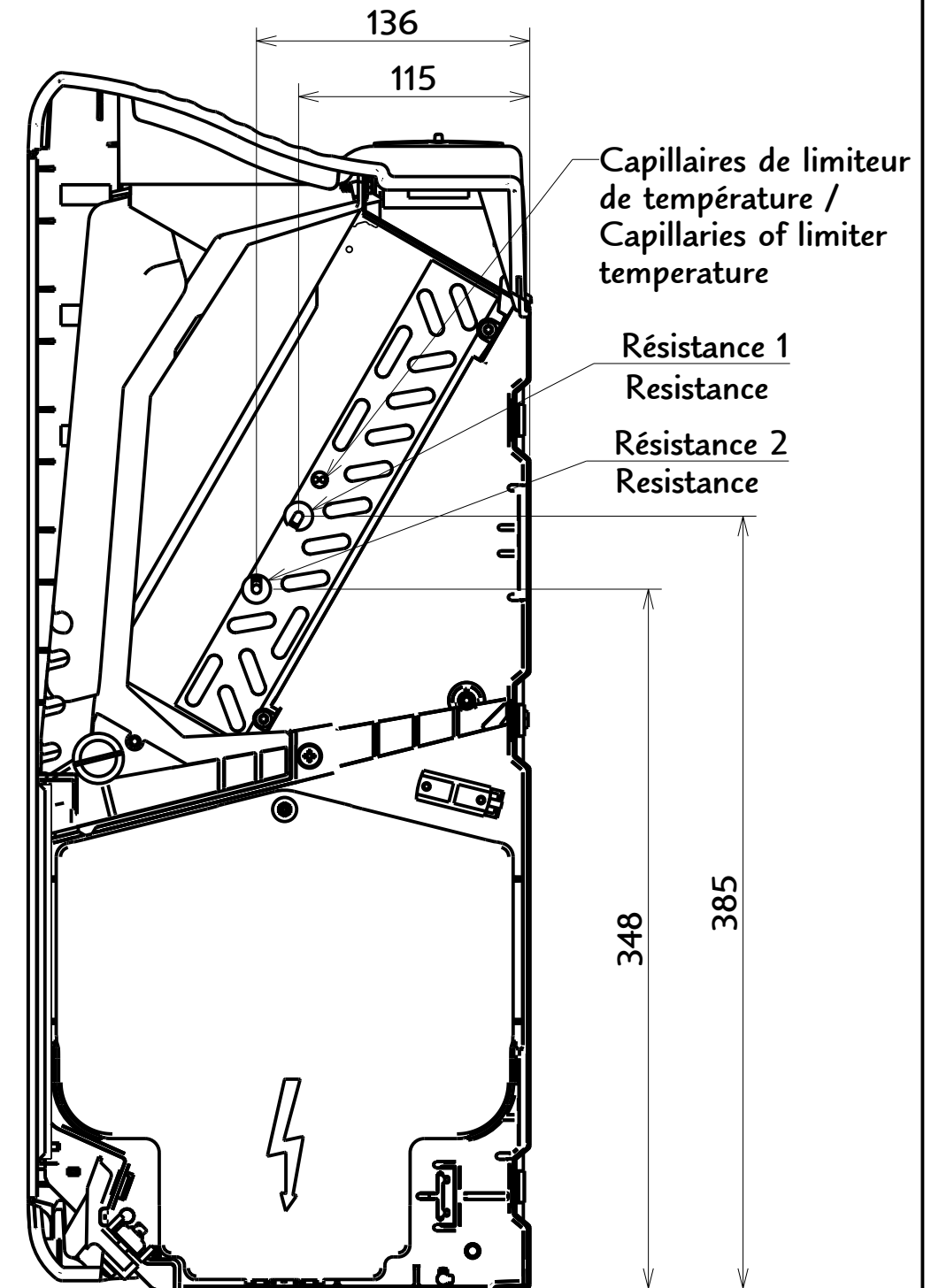
BATTERIE 2T POSITION DES RESISTANCES ( PRISES A GAUCHE ) / COIL 2T POSITION OF RESISTANCE (LEFT HAND CONFIGURATION)
