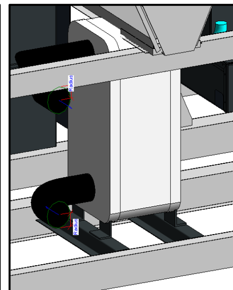
Connectors at Inlet and Outlet Connections of the unit ( Hydronic Kit, BPHE piping and Buffer Tank)
