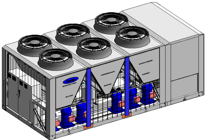
30RB-RBP Revit Family in Project Environment
