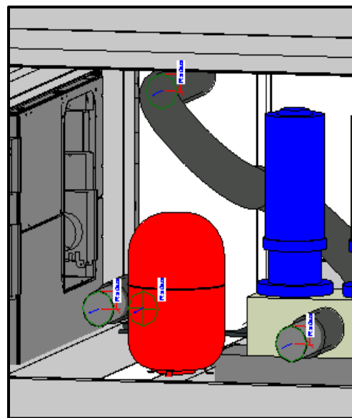
Connectors at Inlet and Outlet Connections of the unit ( Hydronic Kit, BPHE piping and Buffer Tank)
